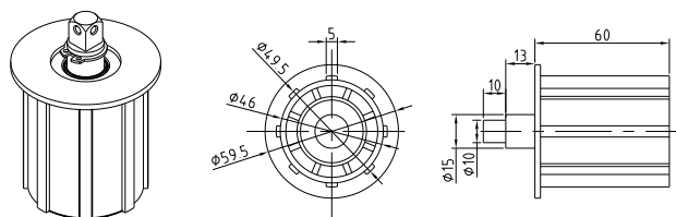
尾塞/idler A1003
