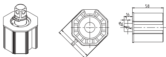
尾塞/idler A1009
