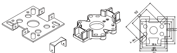
端板/wall plate A3032
