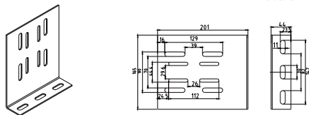
端板/wall plate A3032
