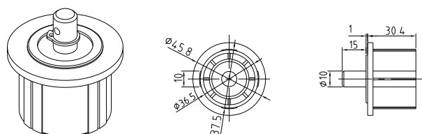
尾塞/idler A1002
