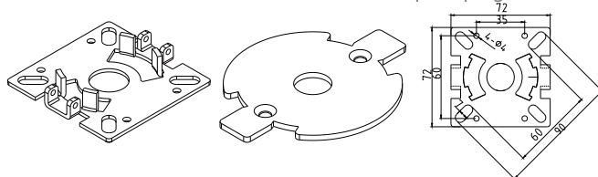
端板/wall plate A3030
