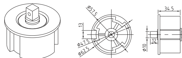
尾塞/idler A1005
