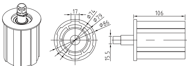
尾塞/idler A1007
