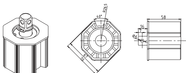
尾塞/idler A1008
