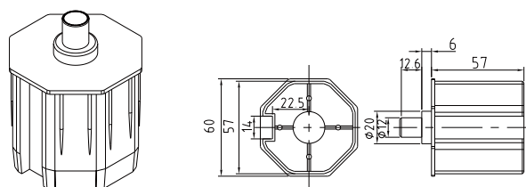
尾塞/idler A1004
