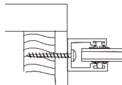
Typical Jamb Details of "U" Type Rails
