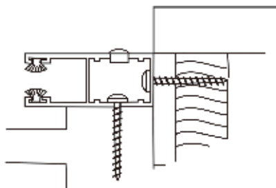
Typical Jamb Details of "A" Type Rails
