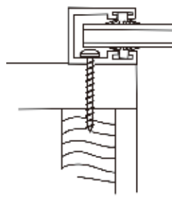
Typical Jamb Details of "U" Type Rails
