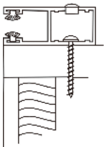
Typical Jamb Details of "A" Type Rails
